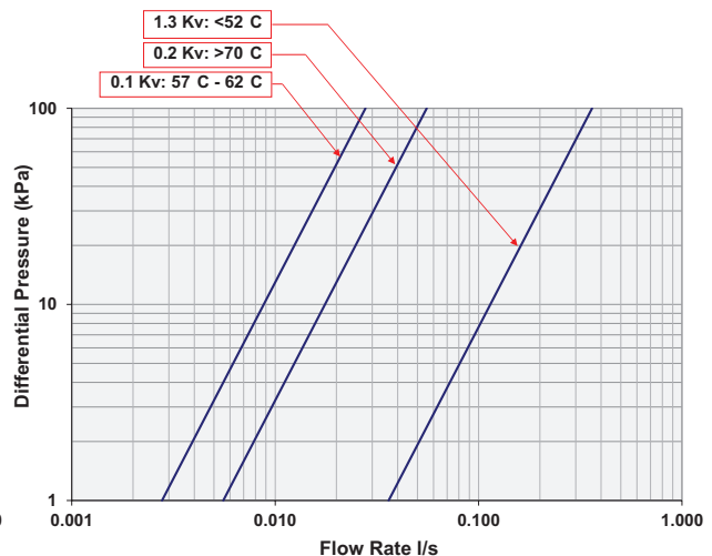
DN15 Standard Flow - D2880 Set Position 57°C
